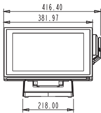
Normal Stand
